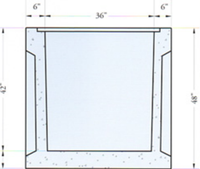
SECTION
