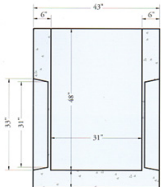
END VIEW
