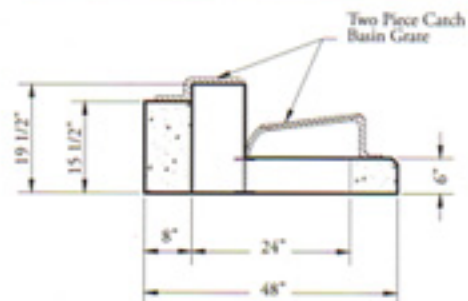
SECTION END VIEW
