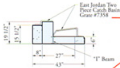
SECTION END VIEW
