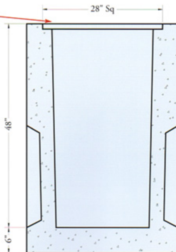
SECTION
