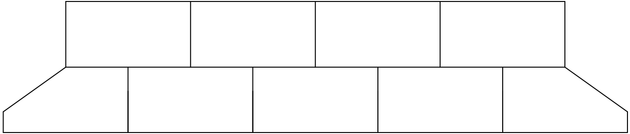
SLOPED STAGGERED JOINT ASSEMBLY
