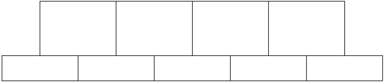
STANDARD STAGGERED JOINT ASSEMBLY
